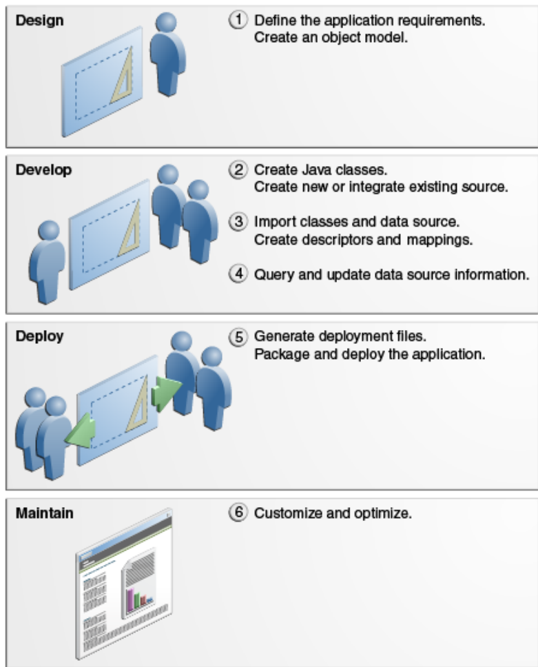
Figure 3-1 EclipseLink Development Process
