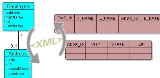
Figure 3–2 EclipseLink Metadata
