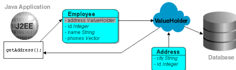
Figure 7-10 Initial Request
