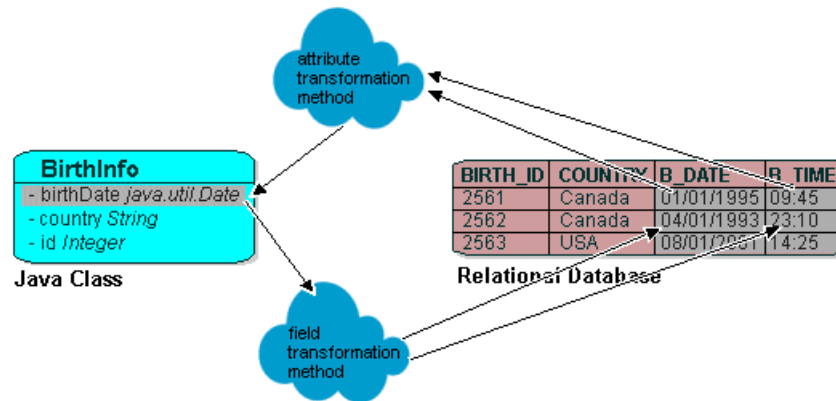
Figure 7-7 Transformation Mappings
