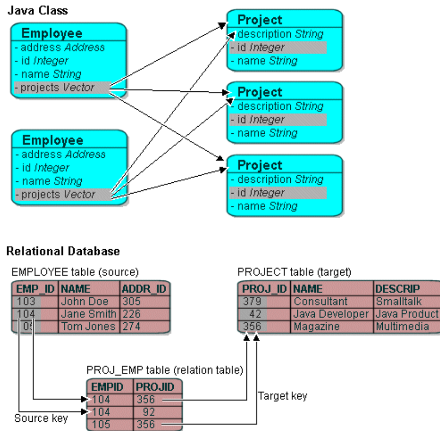
Figure 7–14 Many-to-many Relationships
