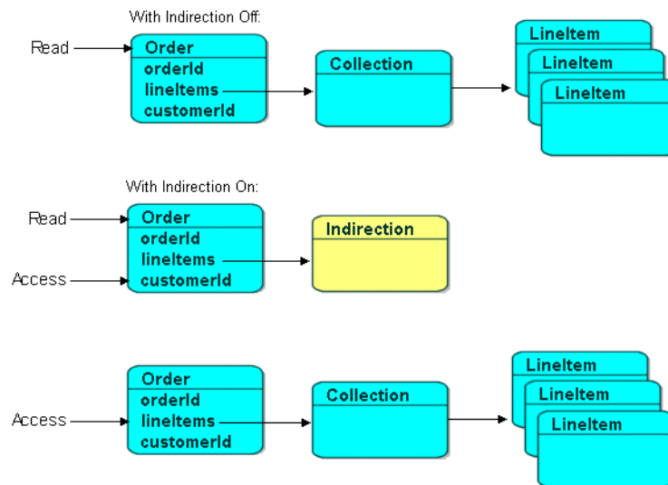
Figure 6–8 EclipseLink Indirection
