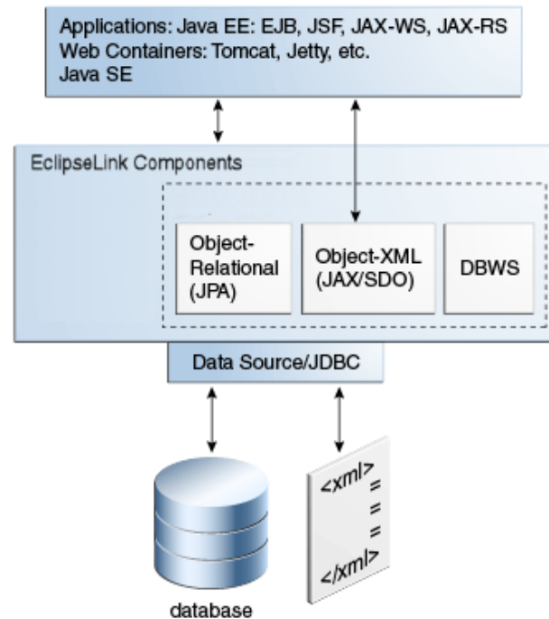
Figure 1-1 EclipseLink Components
