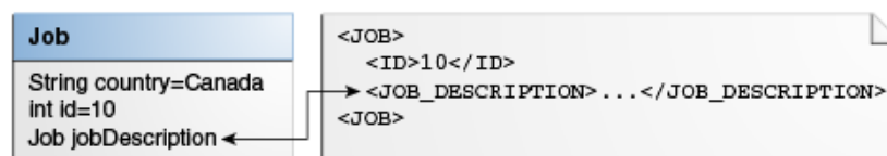
Figure 6–3 Serialized Object Converter (nonrelational)
