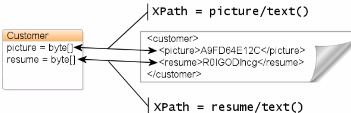
Description of "Figure 4-7 XML Direct Mappings to Different Text Nodes of Different Binary Types"
