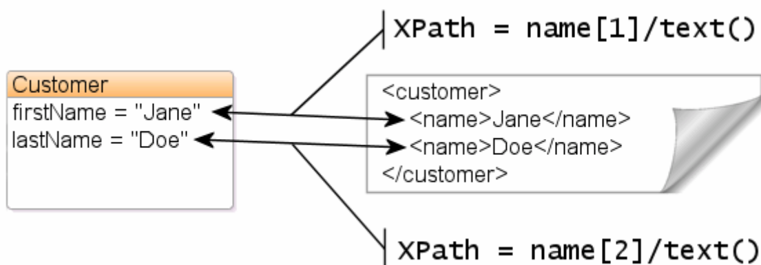
Description of "Figure 4-4 XML Direct Mapping to a Text Node"
