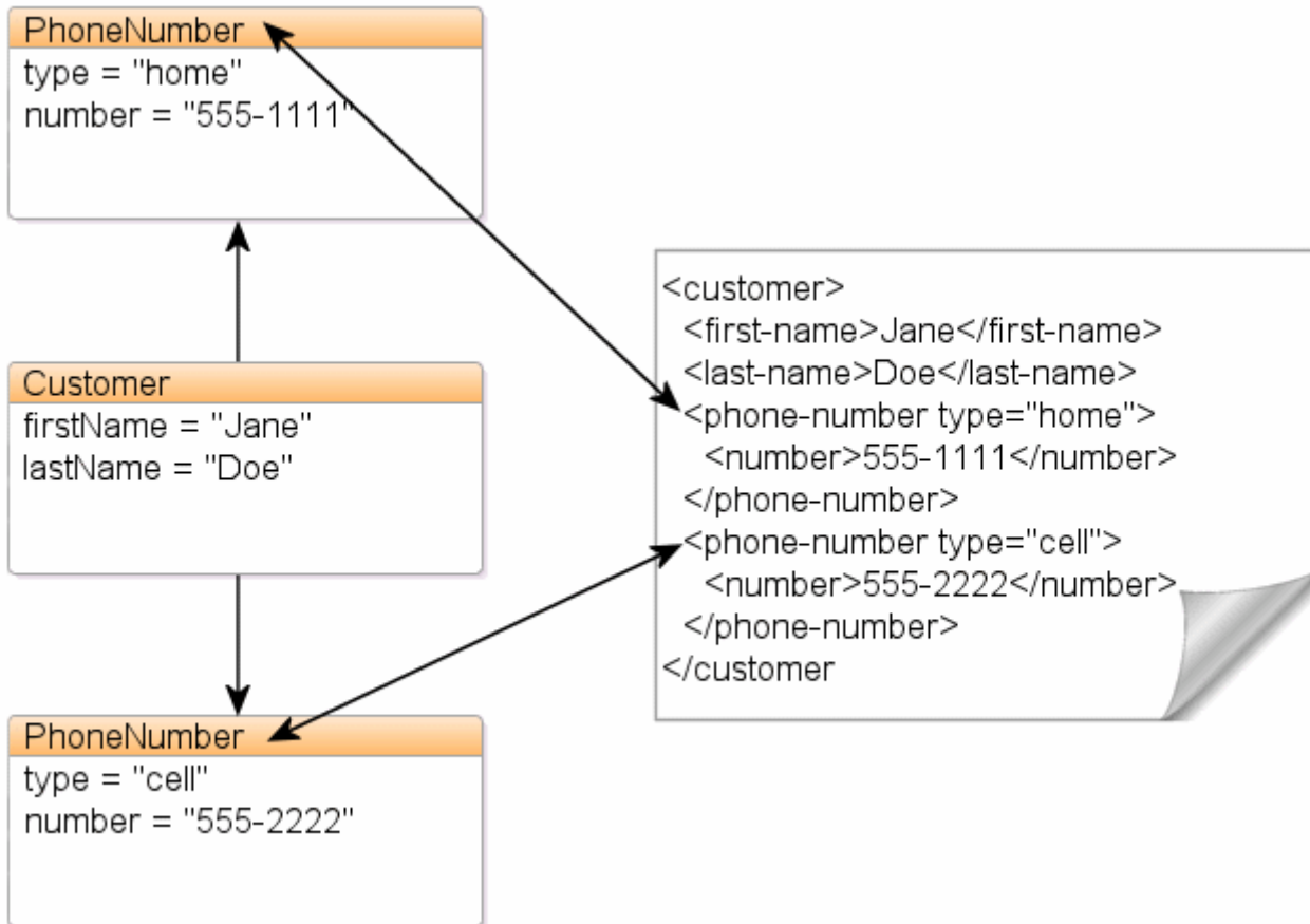
Description of "Figure 6-2 One-to-many Relationship"
