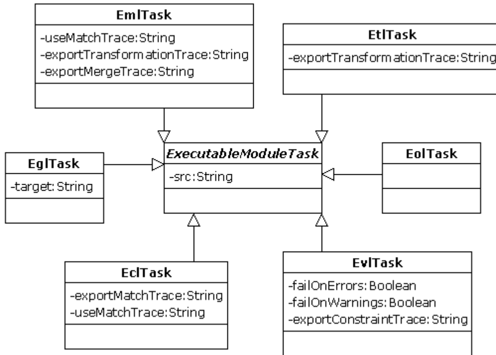
Figure 14.4: Model Management Tasks
