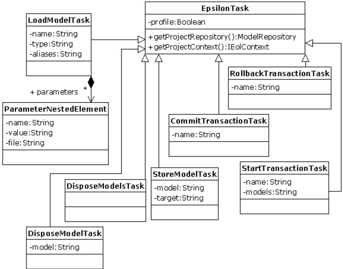
Figure 14.3: Core Models Framework
