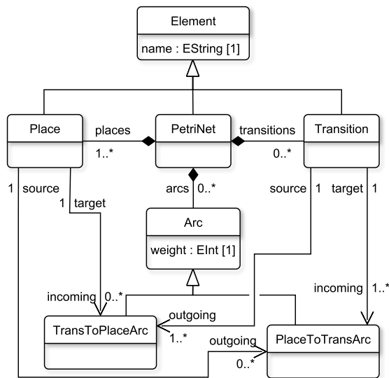
Figure 12.1: PetriNet metamodel
