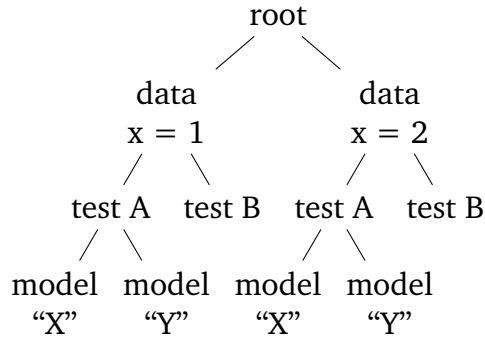
Figure 15.1: Example of an EUnit test tree
