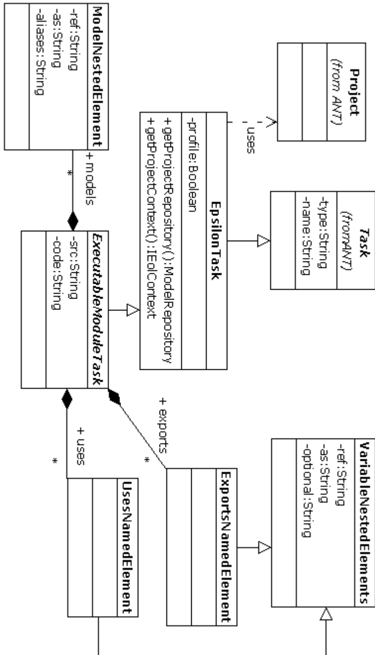
Figure 14.2: Core Framework
