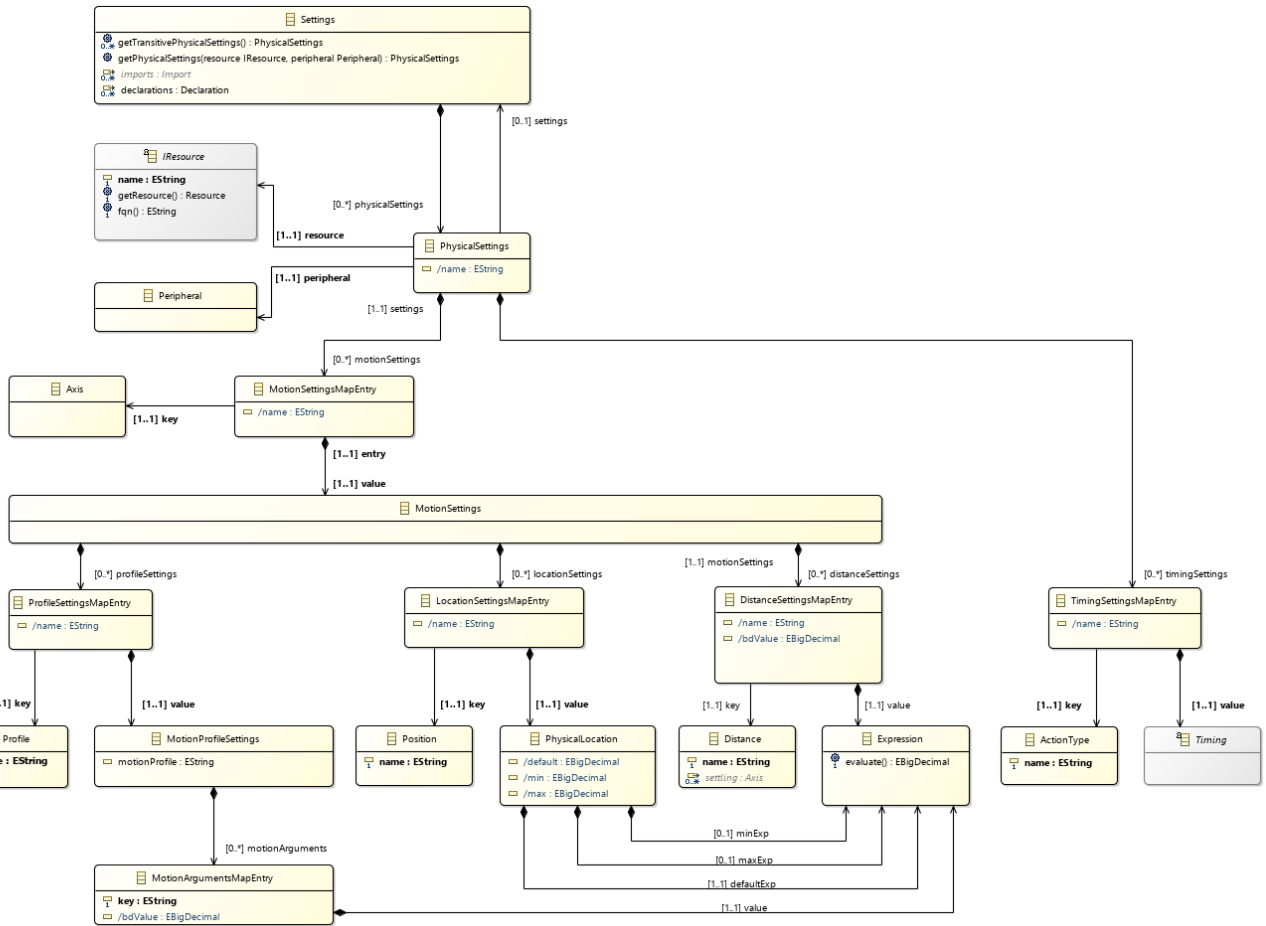
Figure 7. Settings Metamodel
