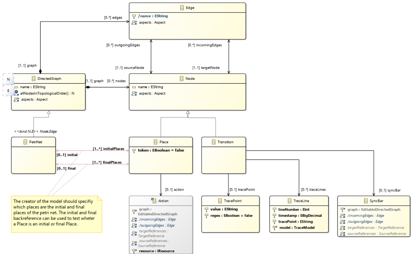
Figure 15. PetriNet Metamodel
