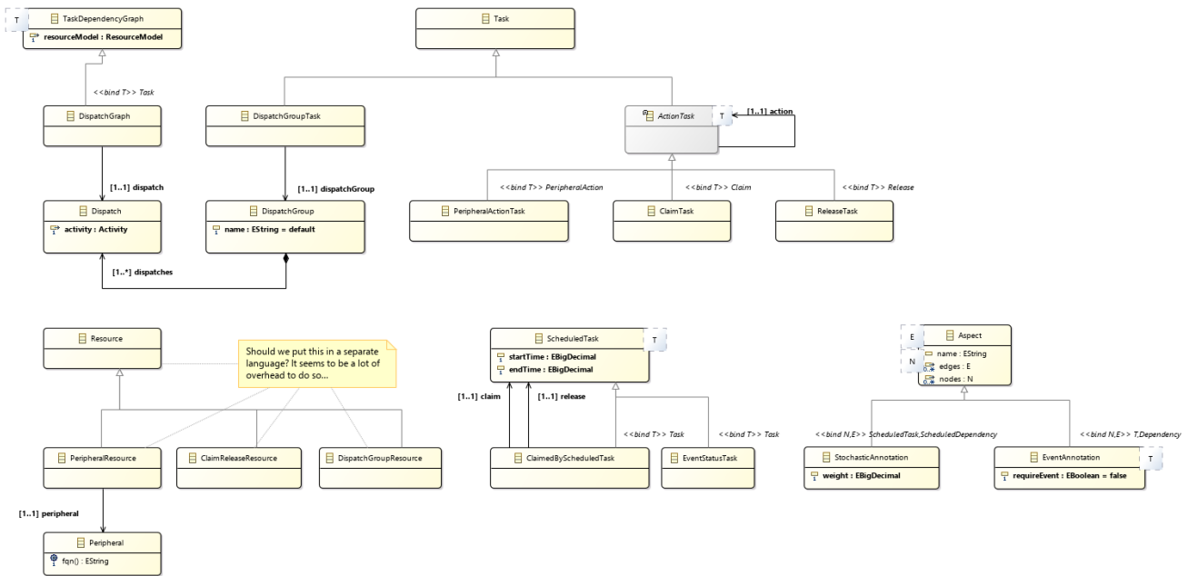
Figure 14. Scheduler Metamodel
