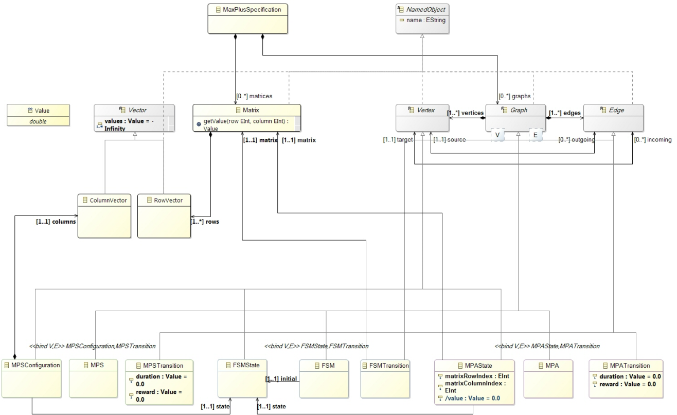
Figure 16. MaxPlus Metamodel
