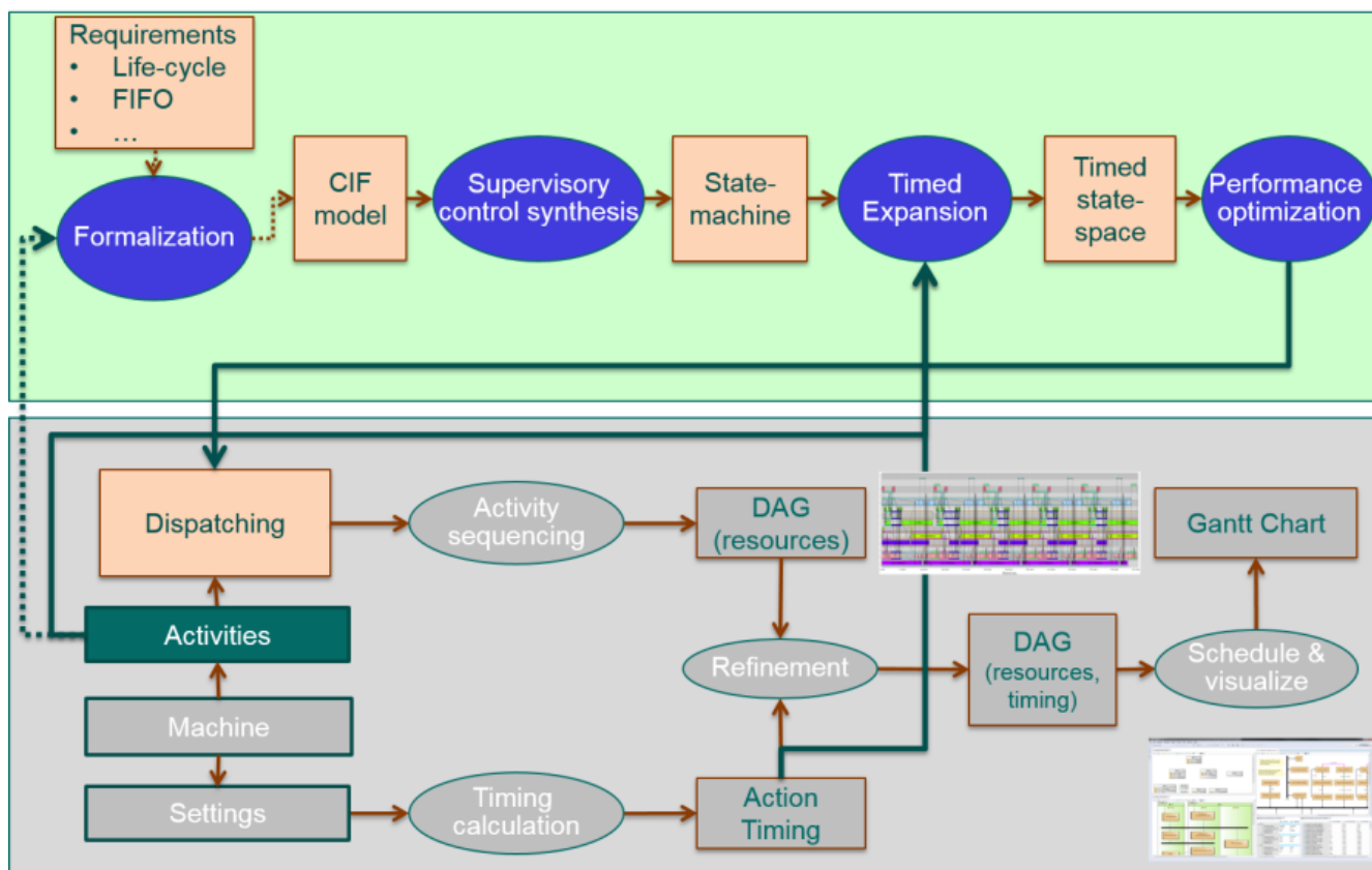
Figure 18. Optimal Makespan/Throughput Scheduling
