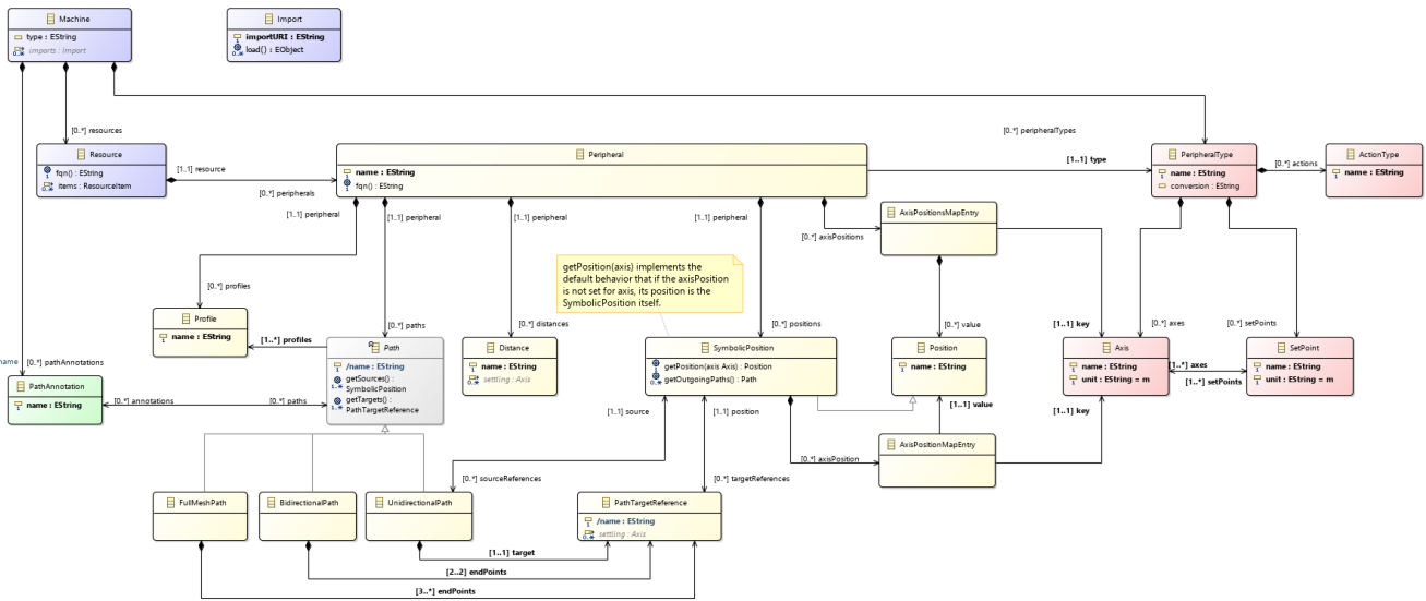
Figure 3. Machine Metamodel
