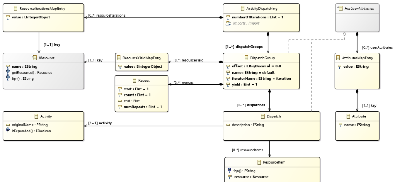
Figure 11. Logistics Metamodel
