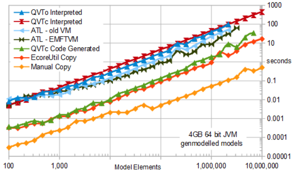
Fig. 5. Performance of the simple Families2Persons transformation.
